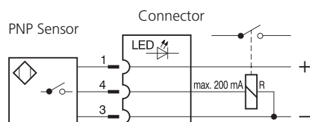
S1 Circuit diagram of the normally - OPEN sensor
